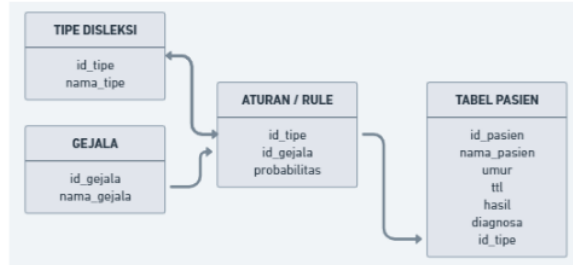
Gambar 6. Relasi Database
